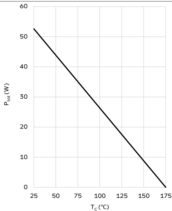
Figure 4. Power derating
